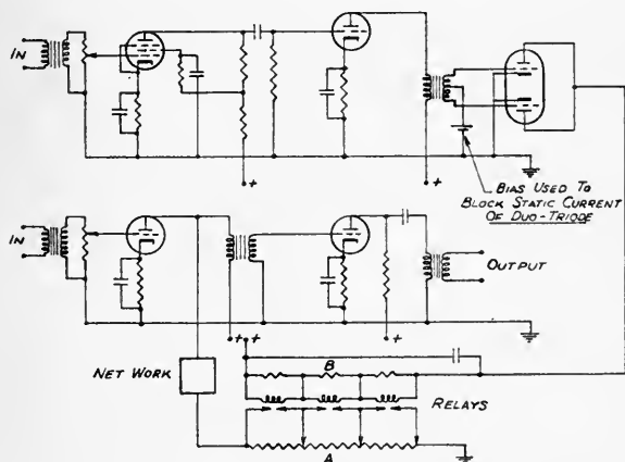
FIG. 4. Mechanical response control.
